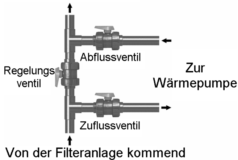
Bypass-Schema
